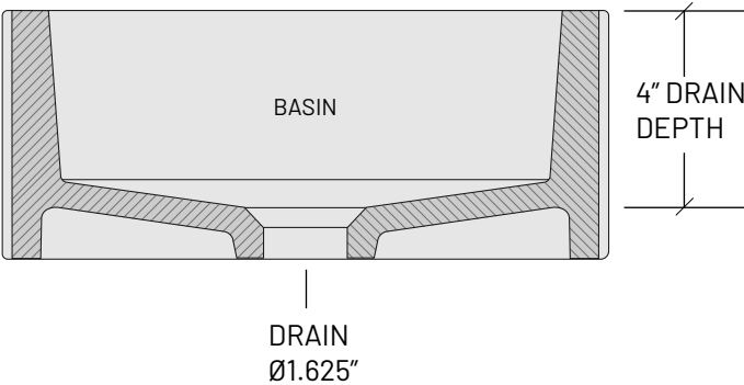
SECTION VIEW / SIDE
