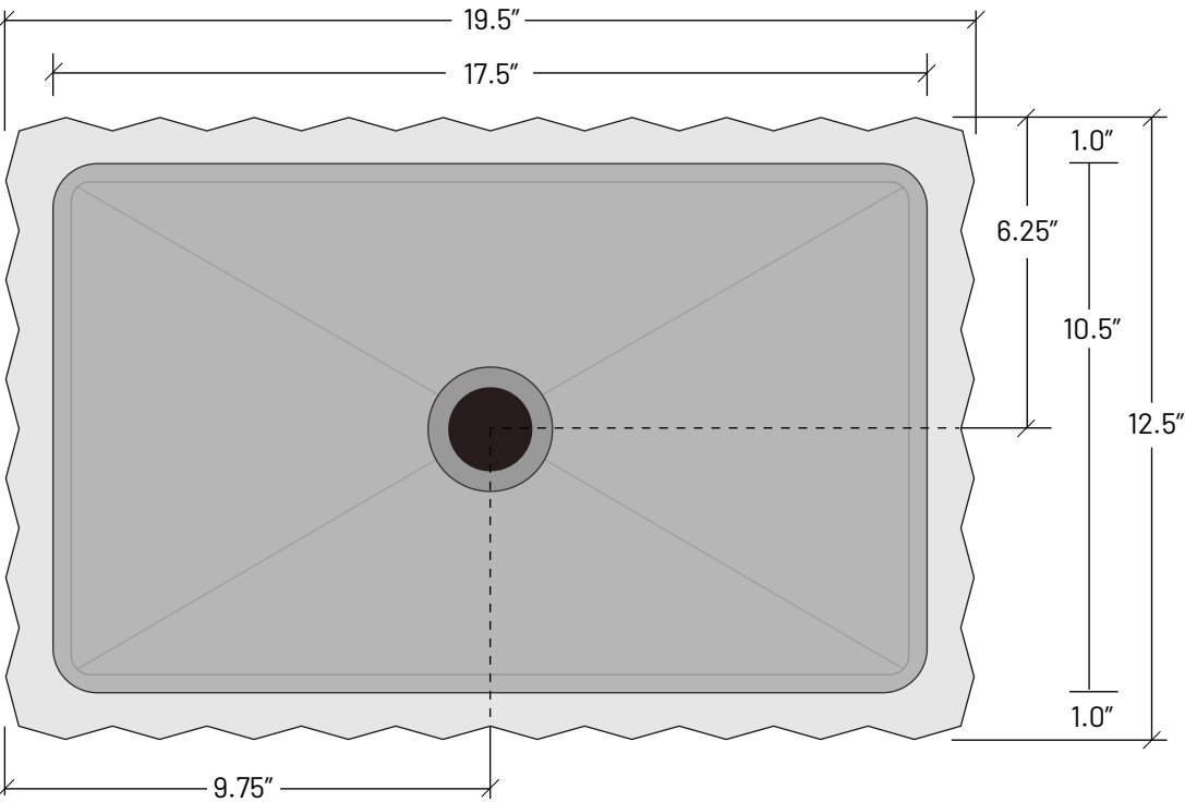
PLAN VIEW
