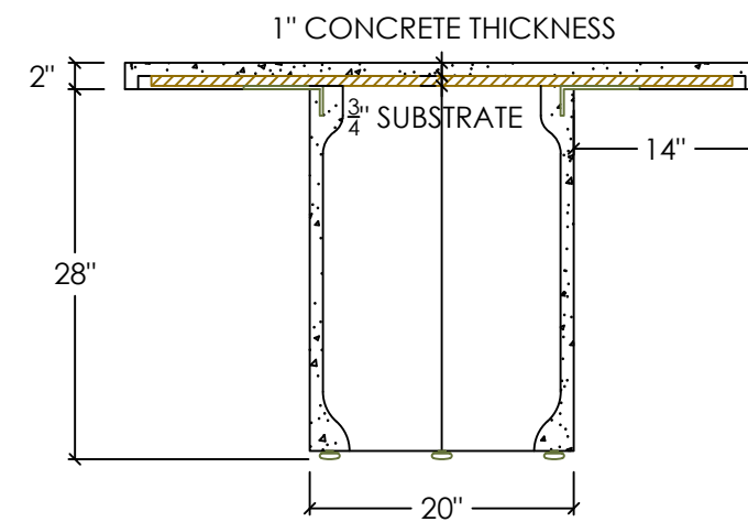
RIGHT SECTION
