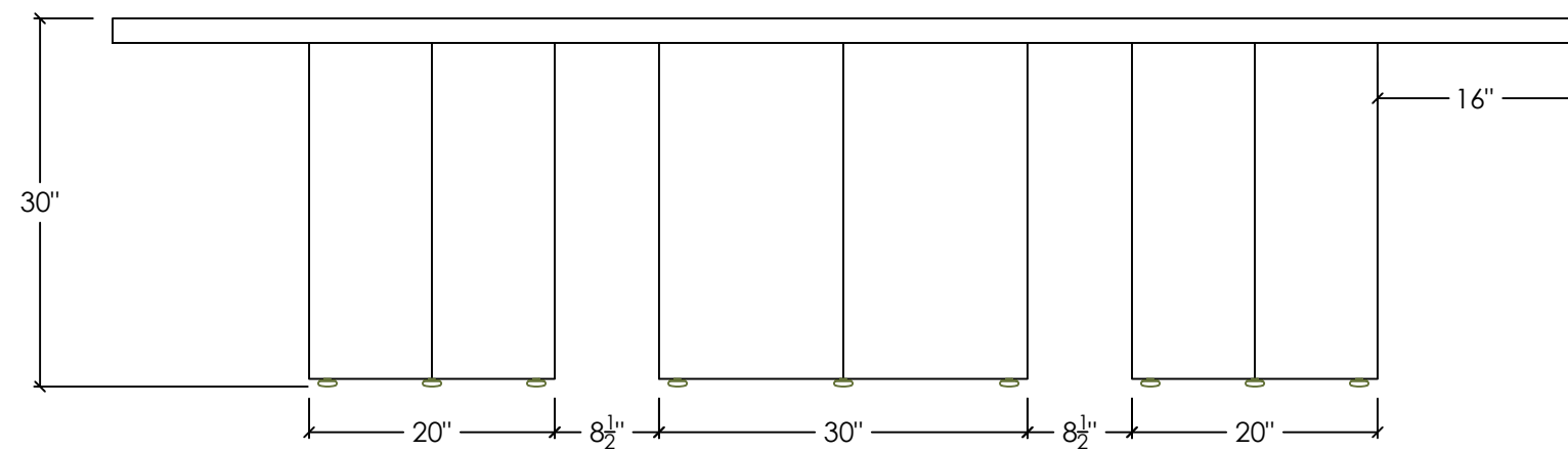
FRONT ELEVATION
