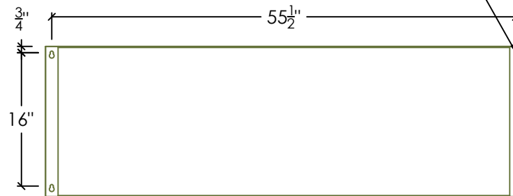
REAR ELEVATION
