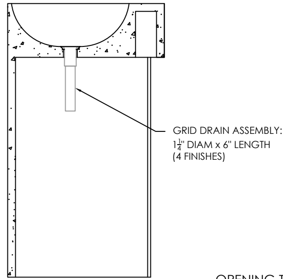
SECTION VIEW
